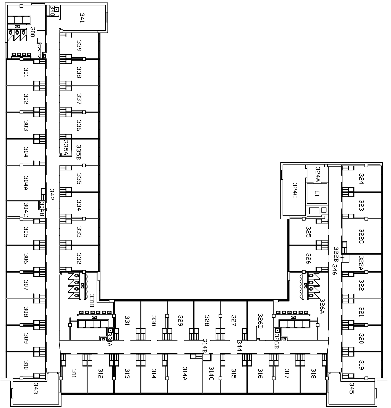
Bldg #026 - Residence Hall, Third Floor
